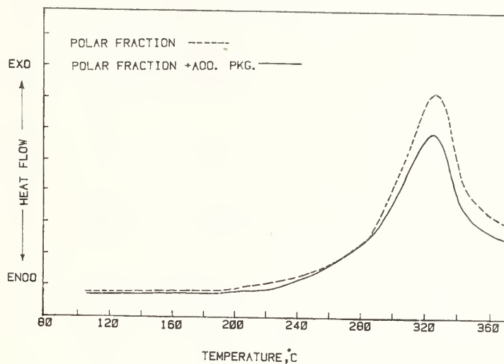
Figure 5. Temperature scanning thermograms of polar fraction from re-refined oil with and without additive package "A".
